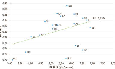
Figure 2. EF (2013 data) – IHD (2013 data) spread for 19 European countries
